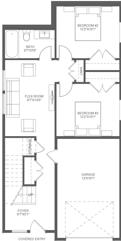
○ LOWER FLOOR PLAN (9' CEILING) LOWER FLOOR AREA: 740.62 Sq Ft GARAGE AREA: 258.87 Sq Ft
