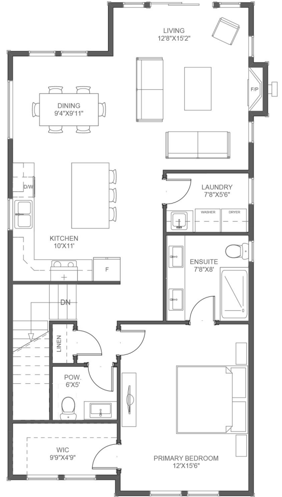
○ MAIN FLOOR PLAN (9' CEILING) MAIN FLOOR AREA: 1,006.16 Sq Ft
