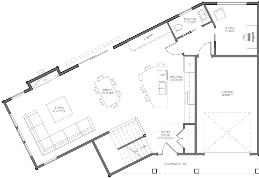
○ MAIN FLOOR PLAN (9' CEILING) MAIN FLOOR AREA: 905 Sq Ft GARAGE FLOOR AREA: 258 Sq Ft
